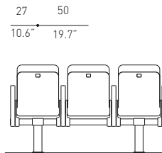
Mod.Compac 800BR
