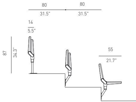
Mod.Compac 801
