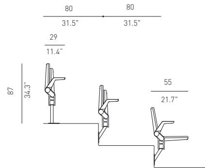
Mod.Compac 801BR
